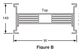
Cross Sections - Plug-In and Indoor Feeder Straight Length (IP-41 and IP-54)
