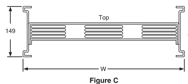
Cross Sections - Plug-In and Indoor Feeder Straight Length (IP-40 and IP-54)
