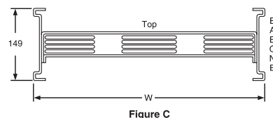
Cross Sections - Plug-In and Indoor Feeder Straight Length (IP-41 and IP-54)
