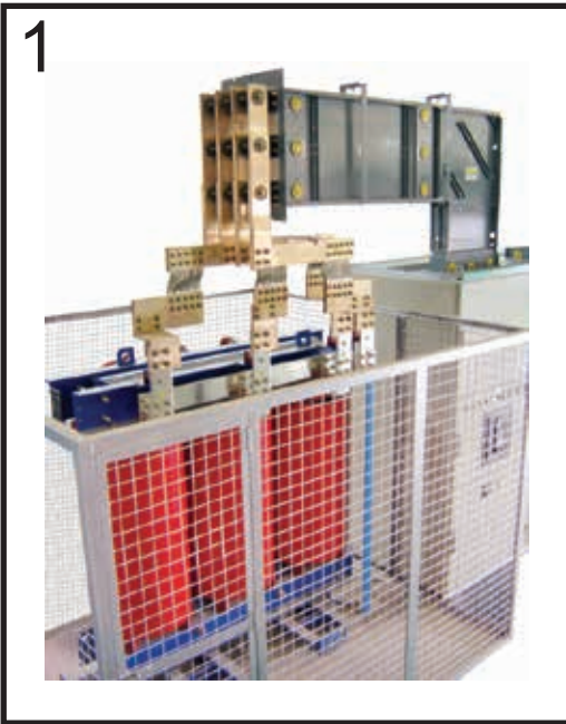
Transformer/Switchboard connection
