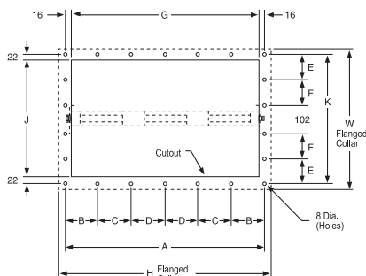
Flanged Collar and Cutout and Drilling Template
