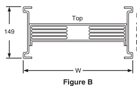
Cross Sections - Plug-In and Indoor Feeder Straight Length (IP-40 and IP-54)
